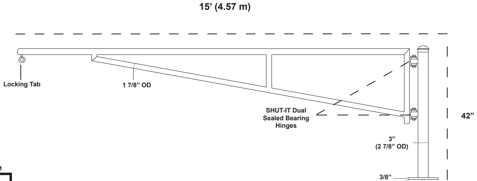
Post & Welded on Plate
